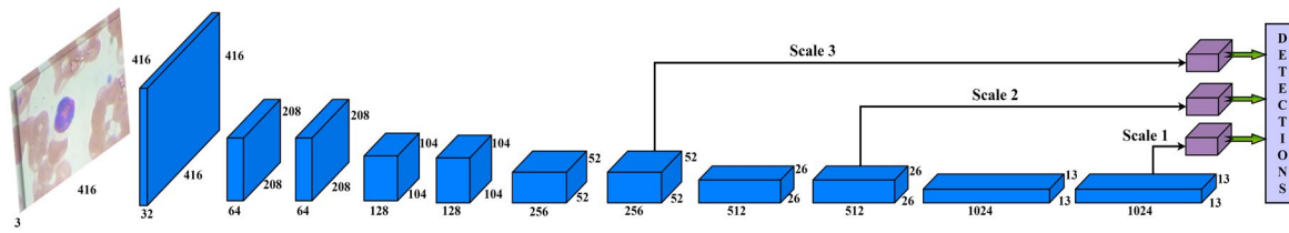
Figure 3. Architecture of the proposed model on processed data.
