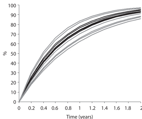
Fig. 8. Growth curves of the different seasonal cohorts for the species of Drepanotrema ( D. lucidum ; D. depressissimum ; D. kermatoides and D. cimex ) inhabiting Paiva pond (black lines) and IMG (gray lines). On the ordinates, the percentage relationship of expected sizes and maximum length, according to the growth model at each time unit (year), is indicated. Cohorts start at “to”= 0.
