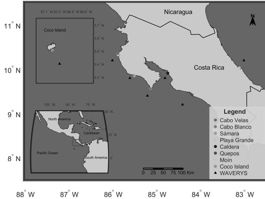
Fig. 1. Spatial distribution of gauges and nodes of reanalysis Waverys.
