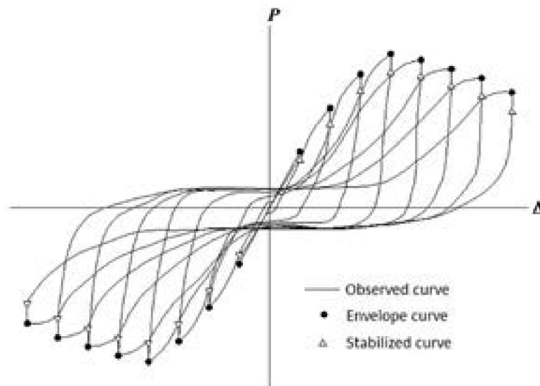
Fig. 3. Envelope curve.
