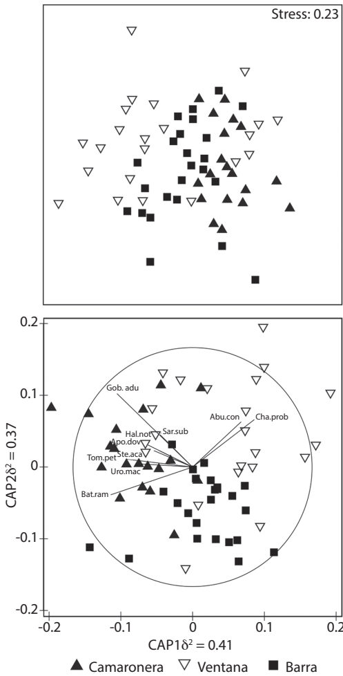
Fig. 1. nMDS and CAP ordinations of tidepool fish assemblages data (ind m -2 ) taken in 2006 at three sites in Gorgona Island, Colombia, Tropical Eastern Pacific. Abbreviations in CAP plot correspond to the first three letters of generic and species names (see Table 1).
