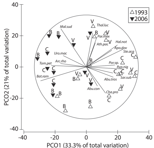
Fig. 2. PCO ordination comparing tidepool fish assemblages from Gorgona Island in 1993 and 2006. Abbreviations correspond to the first three letters of generic and species names (see Table 1). Capital letters indicate sampling localities: (V) Ventana, (C) Camaronera and (B) Barra.
